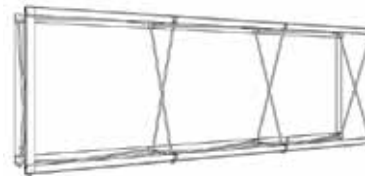
Flat 3w x 1h 2240mm x 770mm
